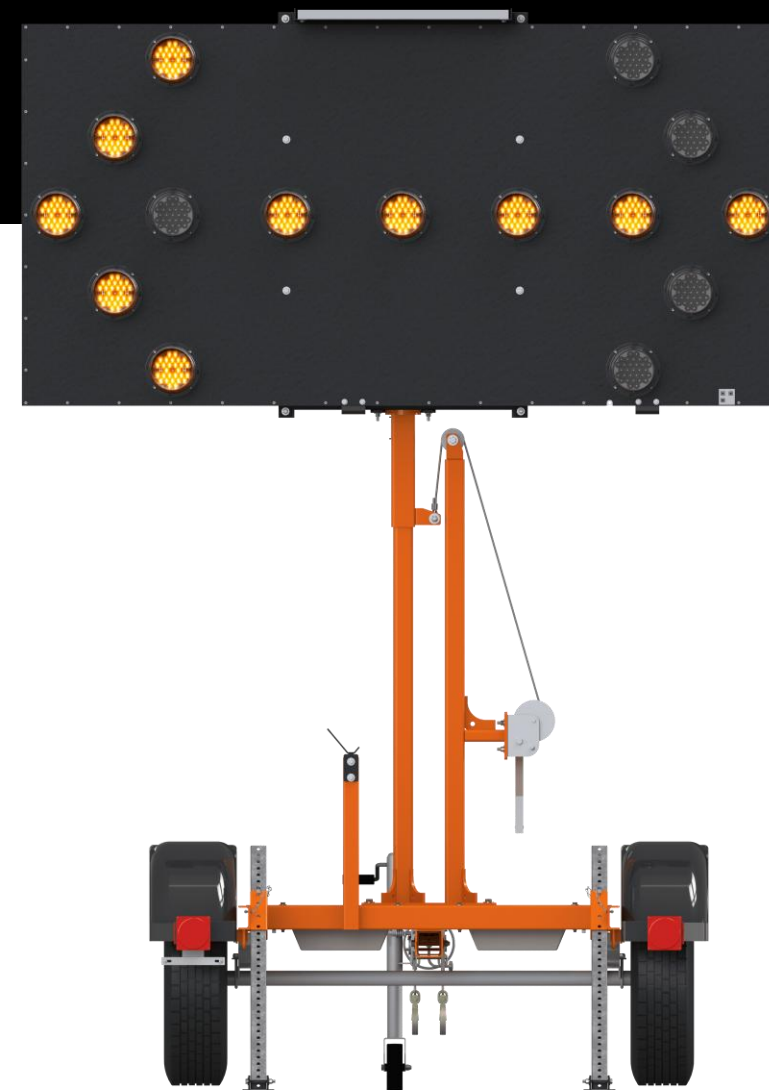
Trailer-Mounted Arrow Board
